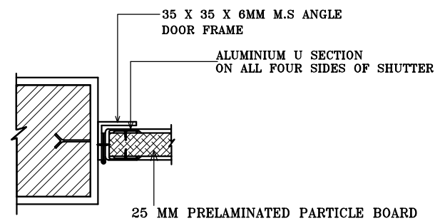
DETAIL AT A
