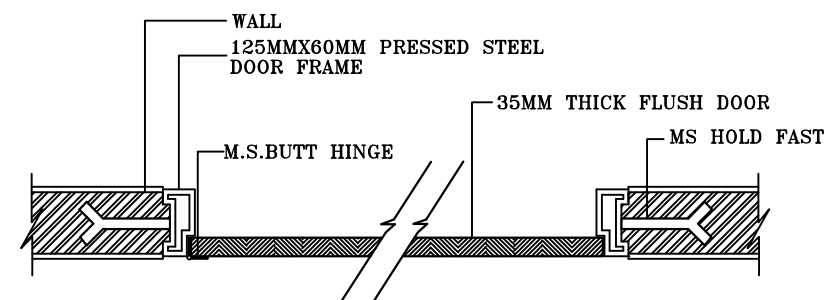
SECTION XX
