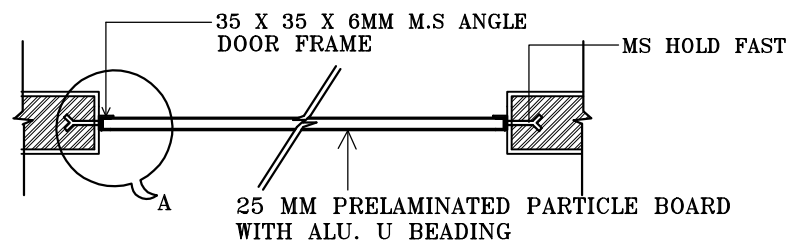
SECTION AT X'-X'
