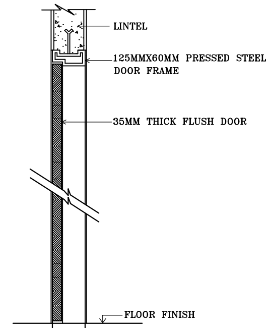
SECTION YY
